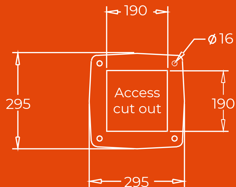
Column Base
